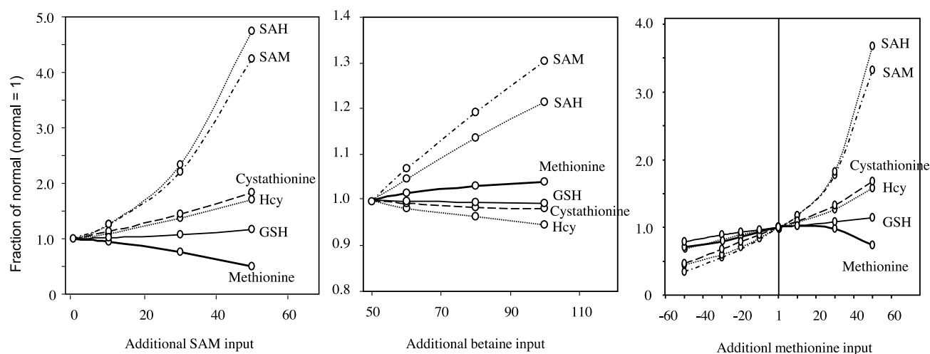
Figure 1. The theoretical effects of increasing methionine input, or the levels of SAM or betaine on the concentrations of other metabolites in the methionine cycle. The model effects of increasing or decreasing methionine input assume that betaine levels are high (as in DS; see Table 1). The model effects of betaine supplementation assume that methionine is unchanged, and that of SAM supplementation assume that betaine is high and methionine is unchanged.
